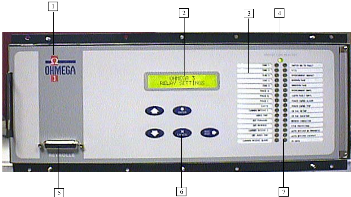
Figure 1–Human Machine Interface (HMI)
